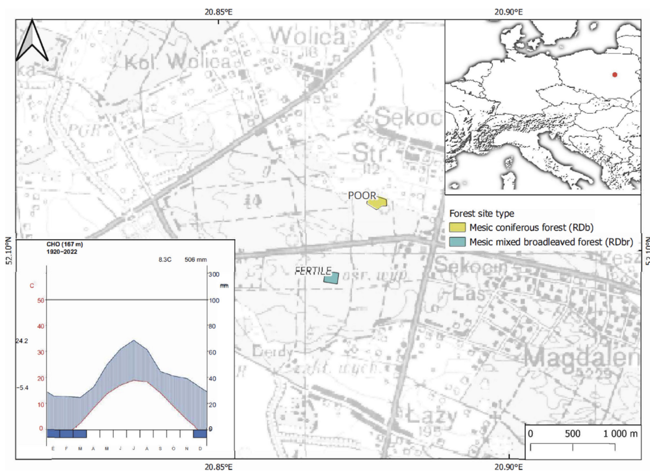
Fig. 1. Location of the study sites (data source: State Forests Information System). Panel in lower left corner: climatic diagram for the area (data source: E-OBS, version 28.0e), RDb and RDbr stand for albic (POOR) and cambic (FERTILE) brunic arenosols, respectively
